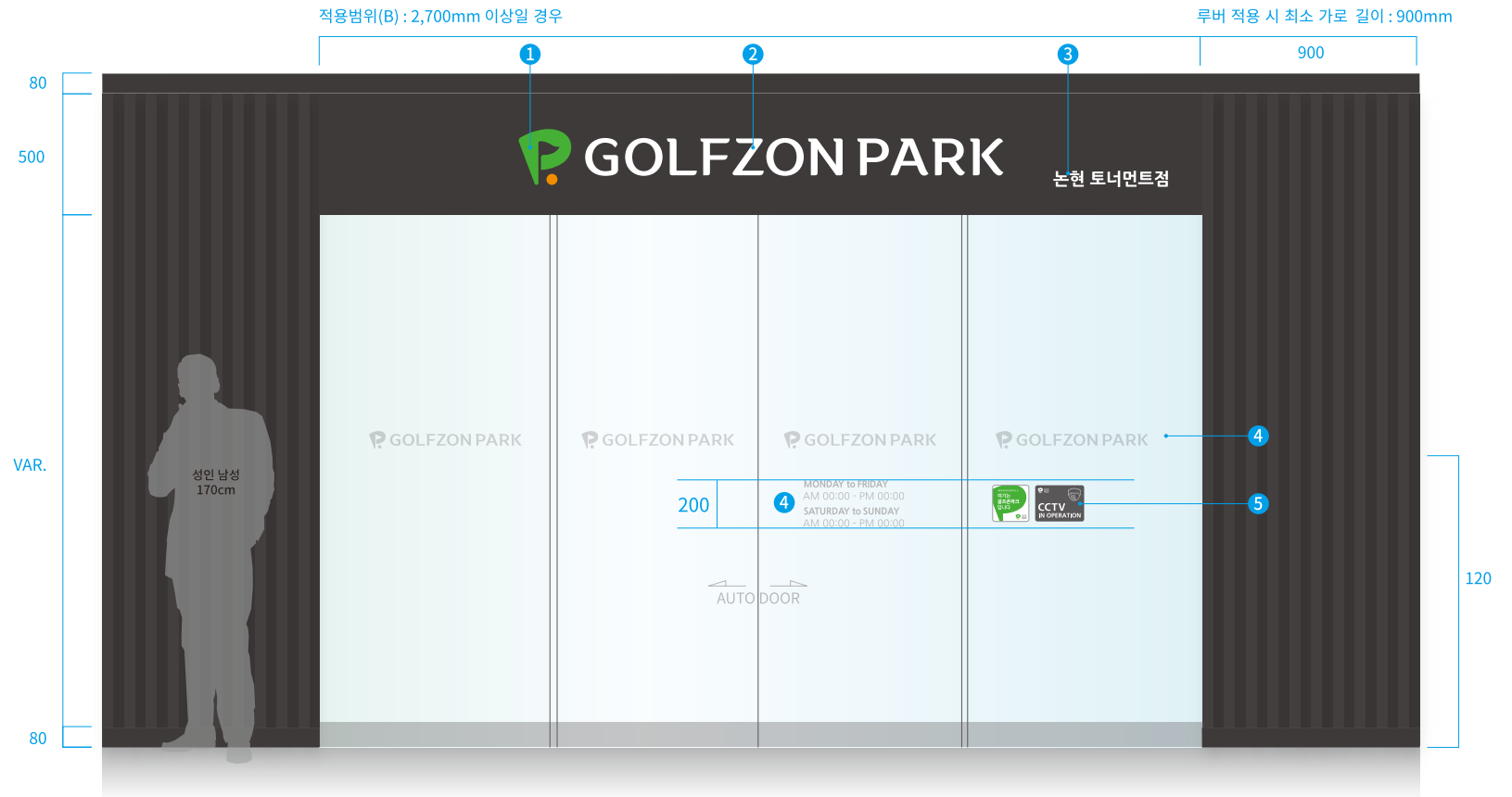
Front View
